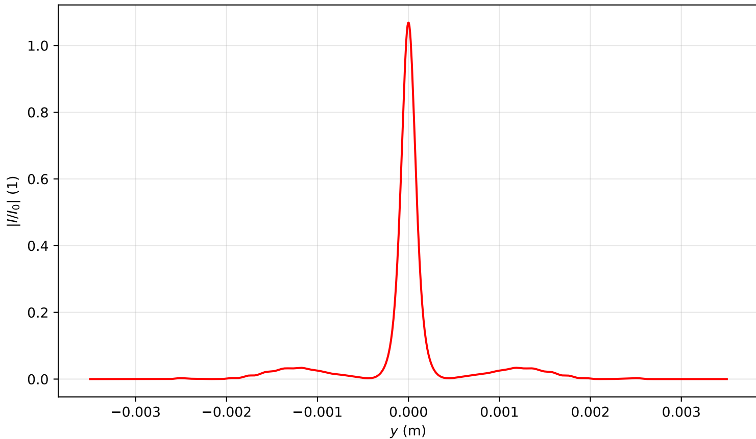
Intensity profile I(x = 0, y, z = 1.274)/I_0 , \text{Pin}=9.0\text{Pcr} , artificial time
